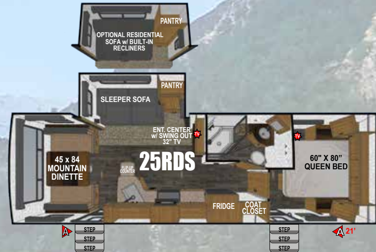
DRY WEIGHT: 7100 ~ FLOOR LENGTH: 27'
